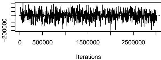
Trace of absdiff.pci
