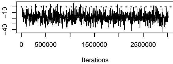
Trace of nodematch.gender
