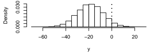
Density of edges
