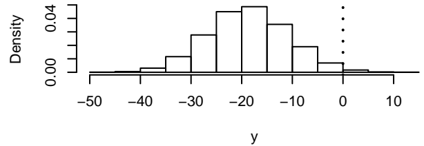
Density of nodematch.gender
