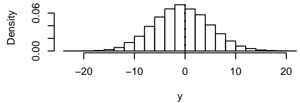
Density of mutual
