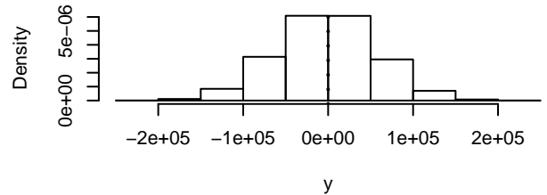
Density of absdiff.pci
